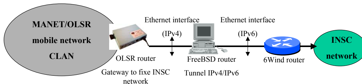
Figure 2-11: INSC Architecture.
