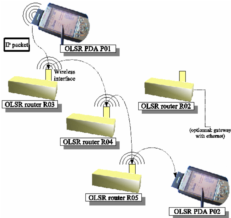
Figure 2-6: MANET/OLSR Demonstrator.
