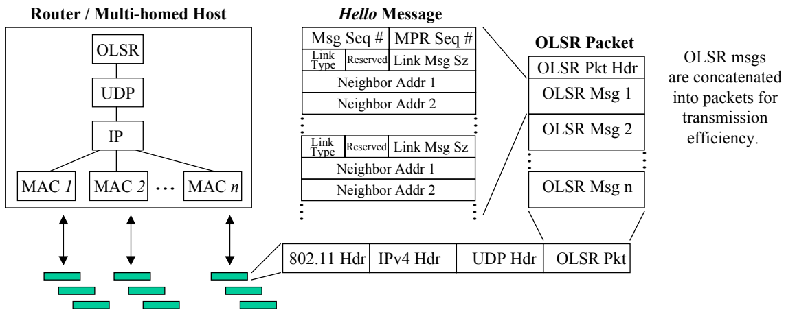
Figure 2-4: OLSR Protocol.
