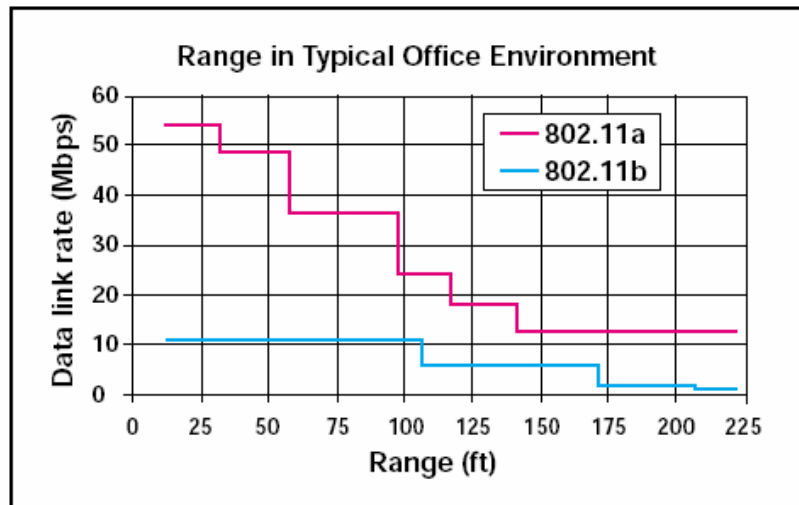
Figure 3-1: WLAN Range.
